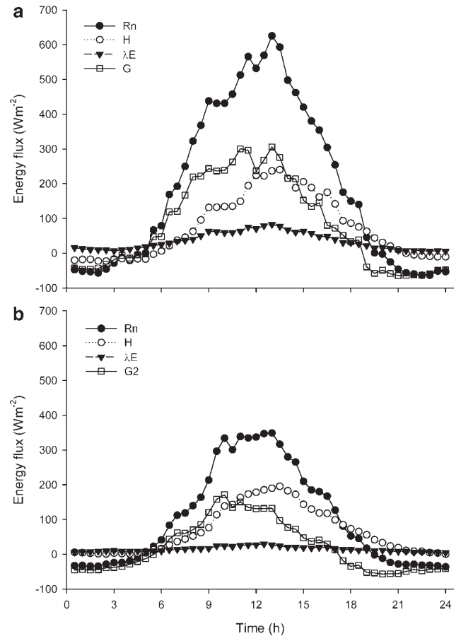
Fig. 6. Same as Fig. 5 but showing net radiation ( R_n ), sensible heat flux ( H ), latent heat flux ( \lambda E ) and ground heat flux ( G ).
